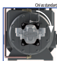
Version HFR Group 4 86,56 cc/rev - Pmax 280 bar -In G 1"1/4 - Out G 1" 1/2
