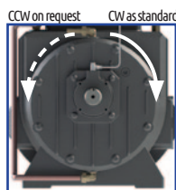
Version PFR Smooth Cylindrical shaft, Ø 40, lenght 90 mm Parallel key UNI 6604
